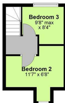
Second Floor Approx. 193.5 sq. feet
